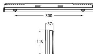
LED Stop/Rear Position/Rear Direction Indicator/Reversing Lamp with Retro Reflector and Number Plate Function
